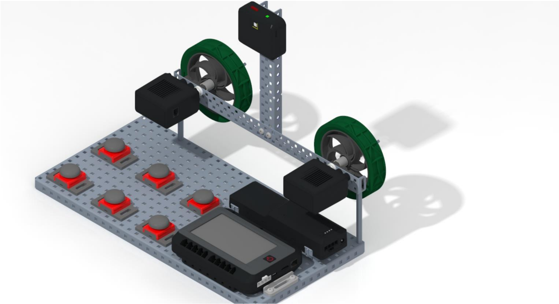
TEST BED - ISOMETRIC
